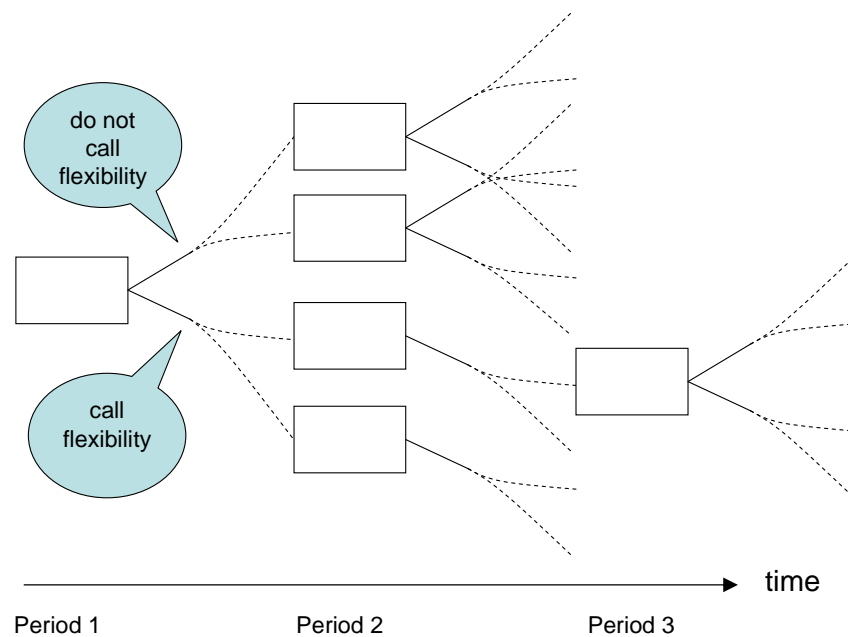
Figure 2-2: Illustration of the explosion of system states when during each period one binary decision (shown with solid lines) can be made, and there is a random event (shown with dotted lines), which affects subsequent decisions and random events. Here the decision can be e.g. to call load flexibility and the random event can be a change in forecast of market price.
